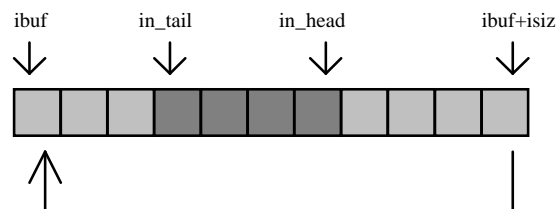
Figure 4.1 Circular ring input buffer
