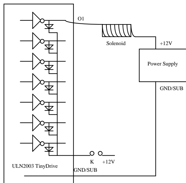
Figure 3.3 Drive inductive load with high voltage/current drivers.
