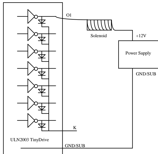
Figure 3.4 Drive inductive load with high voltage/current drivers.
