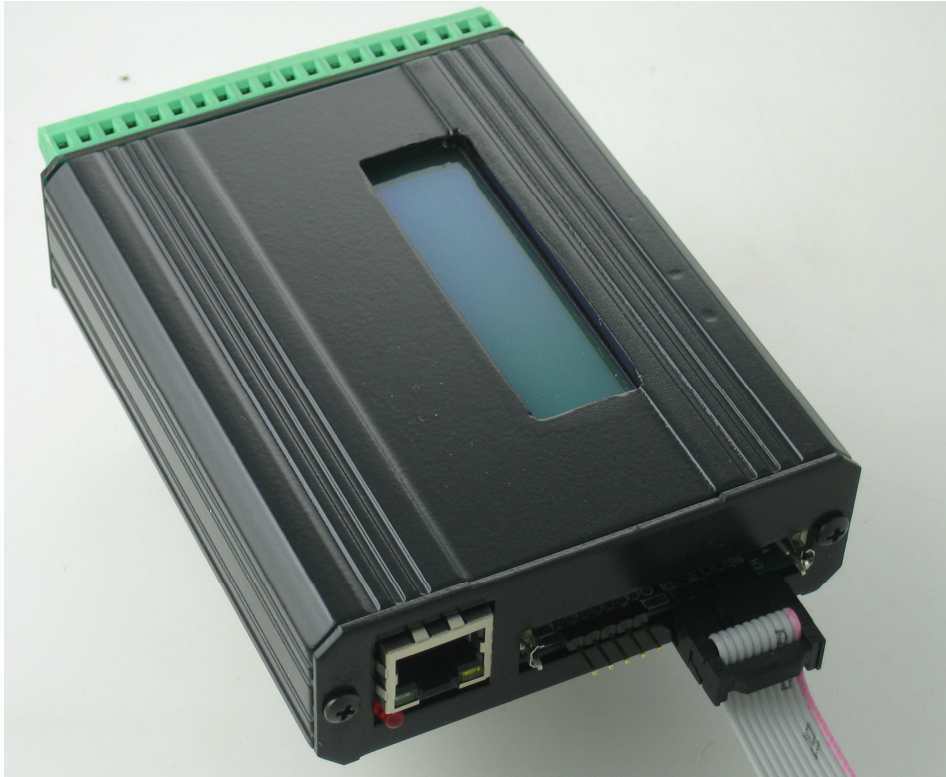
Figure 2.2 DEBUG port for T-Box with enclosure.
