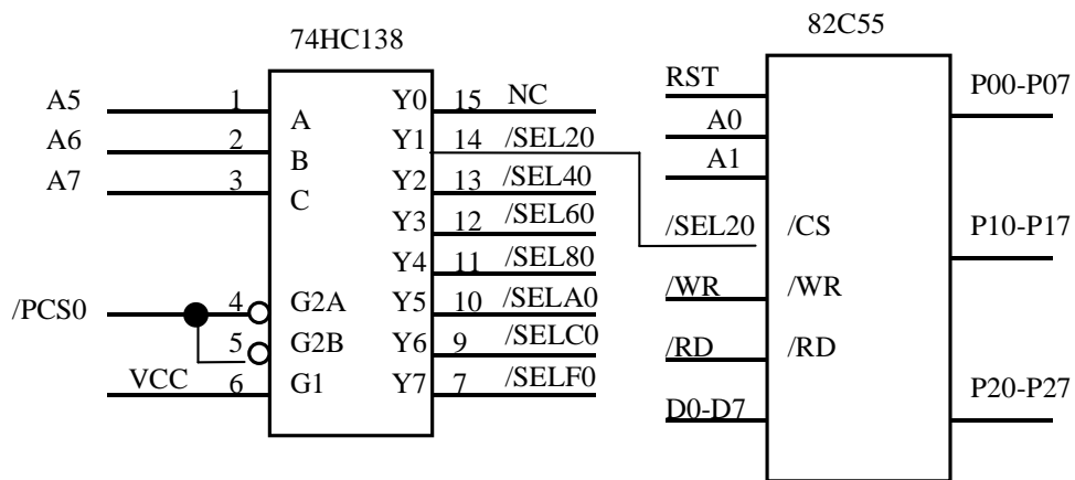
Figure 3.2 Interface the TB to external I/O devices
