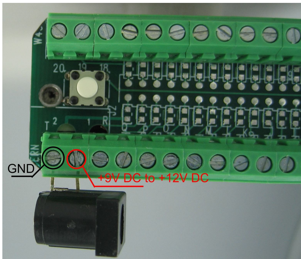
Figure 2.3 Power connection for T-Box with enclosure.
